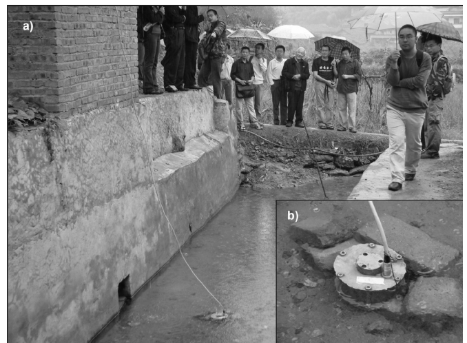
Fig. 3. a) Installation of a submersible flow-through field fluorimeter (GGUN-FL30; Schnegg, 2002) for continuous monitoring of fluorescent tracer concentrations at a karst spring in the Qing Muguan catchment, Chongqing province, China; b) detail of the instrument (photos: N. Goldscheider)
